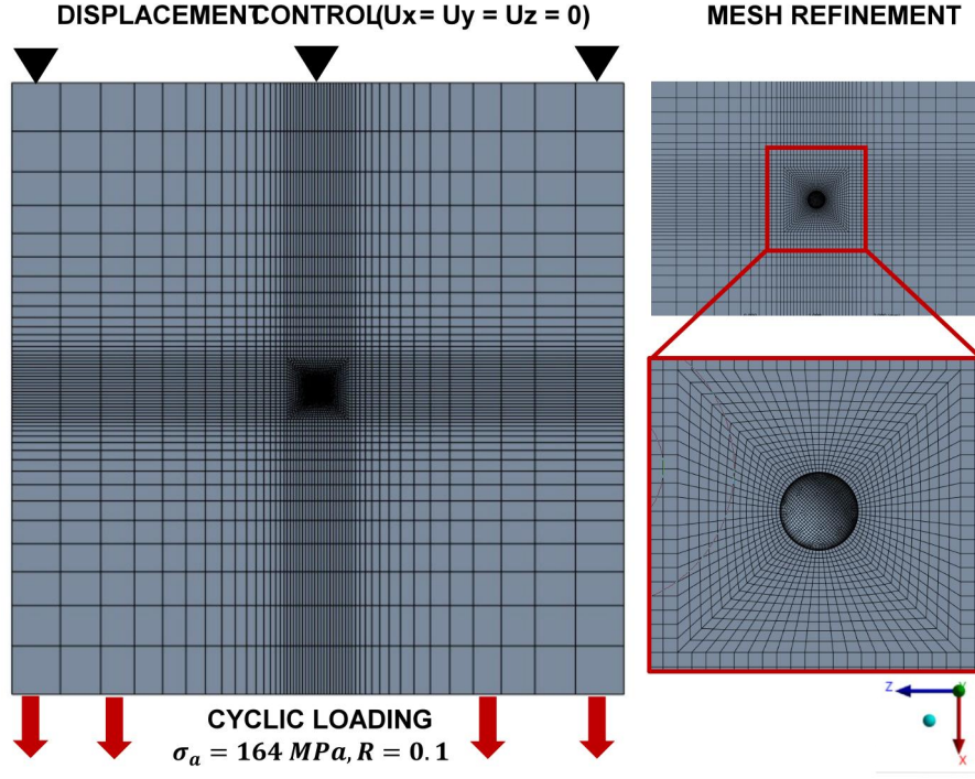
Figure 4. Boundary conditions and meshing strategy used for the benchmark model.
