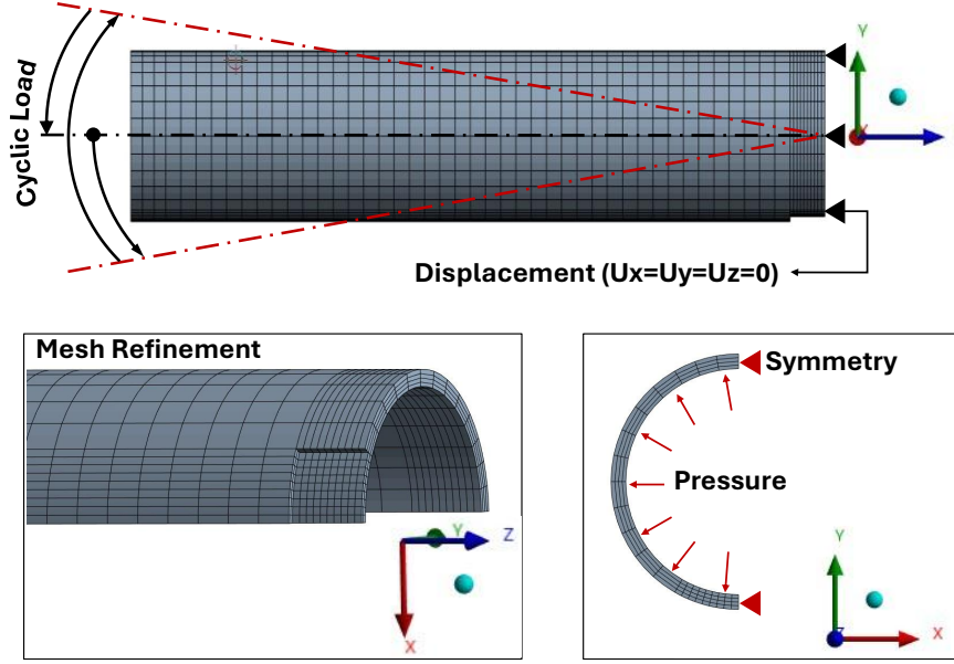
Figure 9. Applied Boundary Conditions
