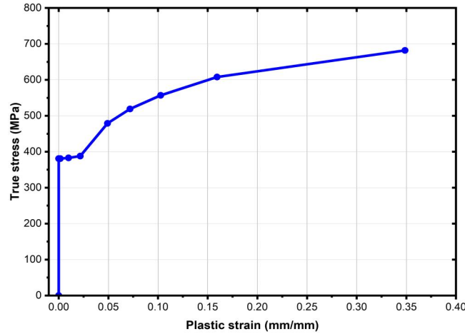
Figure 5. Literature-derived true stress–plastic strain input curve for API 5L X52 steel, adapted from Arumugam, Karuppanan and Ovinis (2020).
