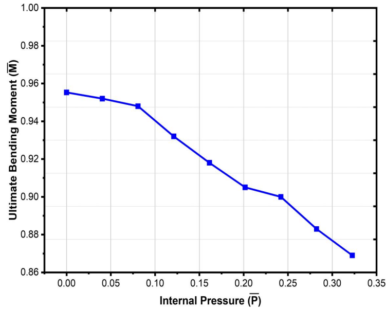
Figure 15. Effect of internal pressure on normalized ultimate bending capacity for l/D = 1 and d/t = 0.5 .
