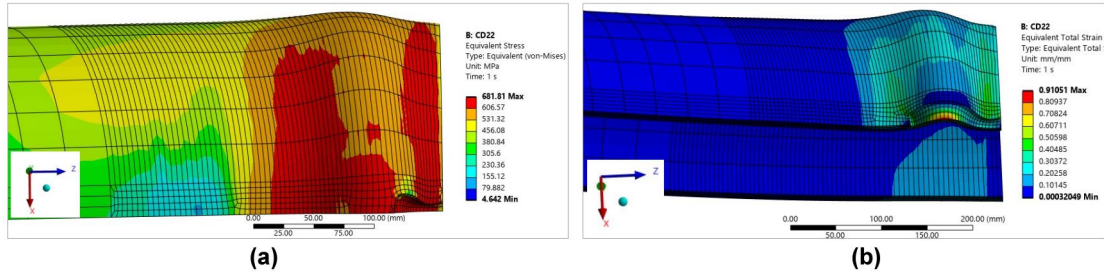
Figure 11. Local buckling mode of the corroded pipe at the ultimate bending capacity: (a) von Mises stress distribution; and (b) total strain contour
