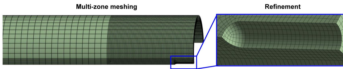
Figure 8. Meshing strategy
